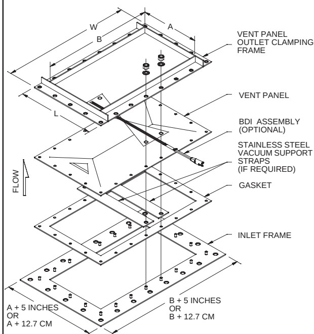
Rectangular and Square Vent Panel / Frame
